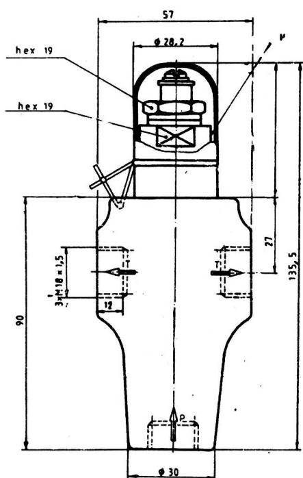
Fig.6.Supape reglabile ,cu surub cu locas hexagonal (S)
